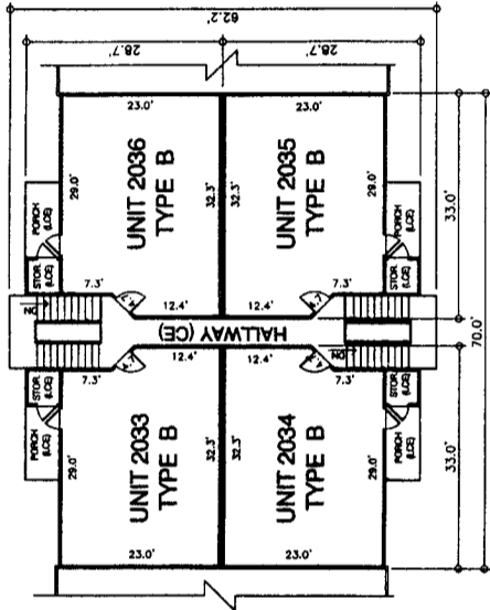
3RD FLOOR
