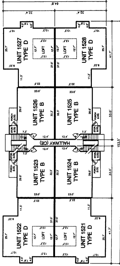
2ND FLOOR
