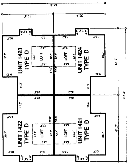
2ND FLOOR
