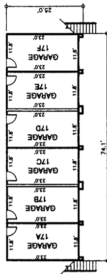
1ST FLOOR
