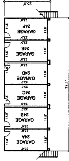
1ST FLOOR
