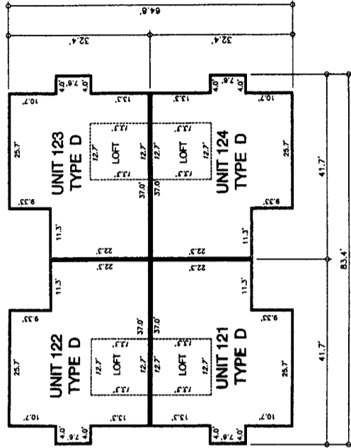
2ND FLOOR
