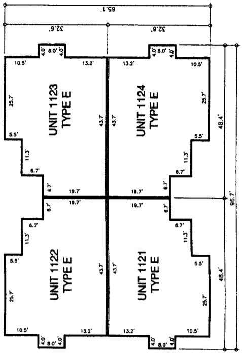
2ND FLOOR
