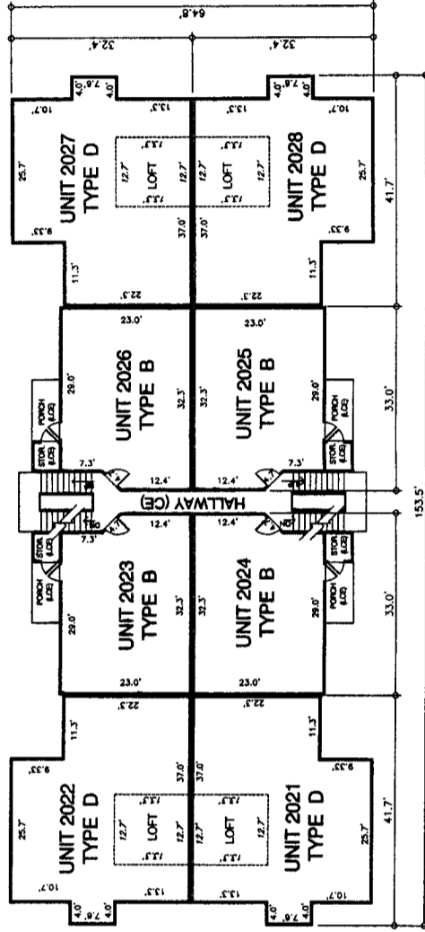
2ND FLOOR
